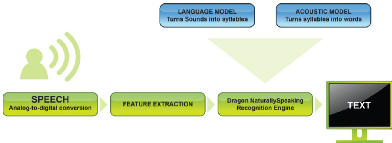
Fig. 1 How Speech Recognition Works
